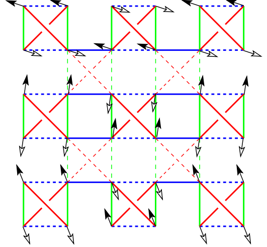
FIG. 16. (Color online) Noncollinear layered state projected along the x axis. The normal of the layers is parallel to the z axis. Frustrated bonds are shown as dashed lines.
