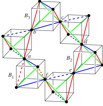
FIG. 15. (Color online) A fragment of a collinear state. Frustrated bonds are shown as colored dashed lines.
